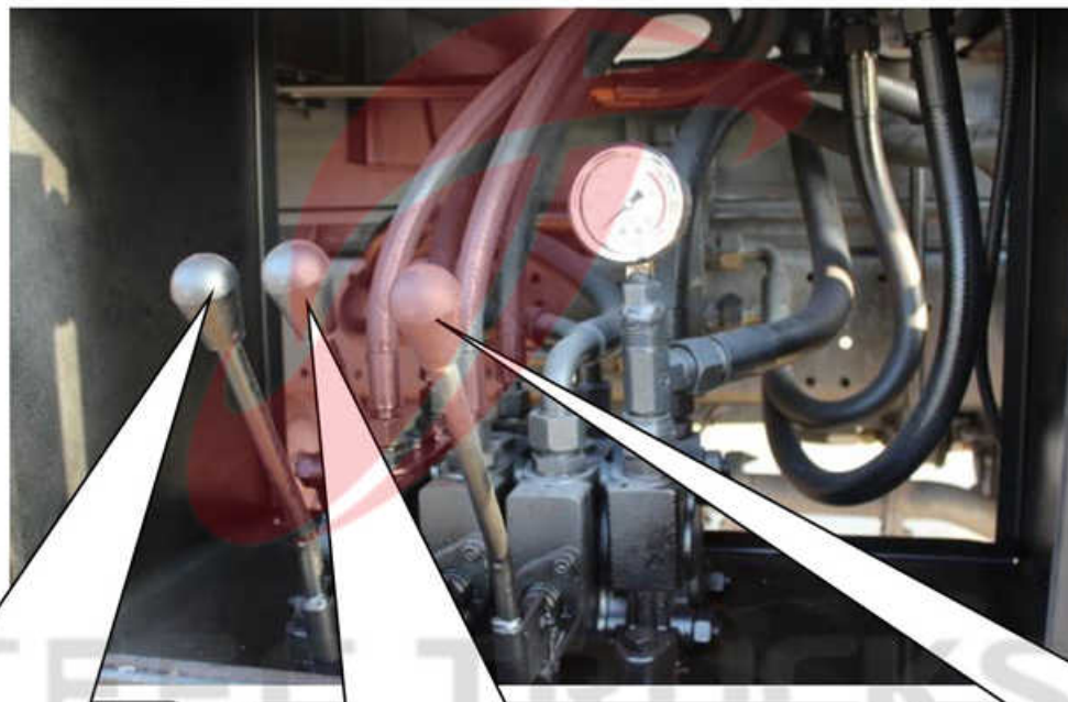
Joysticks two: Control right side hydraulic leg
